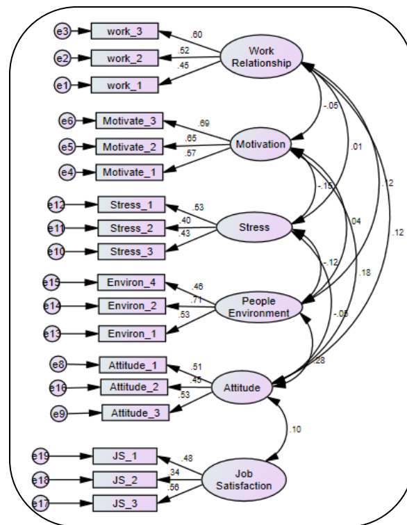
Figure 1: CFA of Measurement Model –Attitude towards Work– Full Fledged Study.
